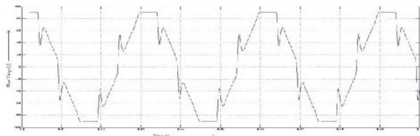
(c) Phase voltage V_{in} .
