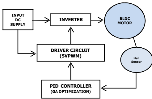
Fig.1.Overall architecture of the proposed system.
