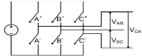
Fig.5. A basic three phase inverter.
